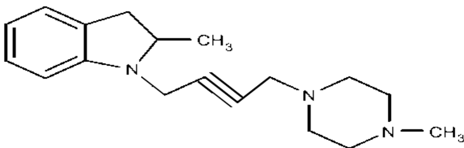
Figure 24: 2-methyl-1-[4-(4-methylpiperizin-1-yl)but-2-yn-1-yl]-2,3-dihydro-1H-indole.
